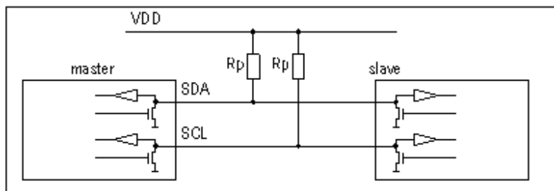
Both bus lines, SDA and SCL, are bi-directional and therefore require an external pull-up resistor.
